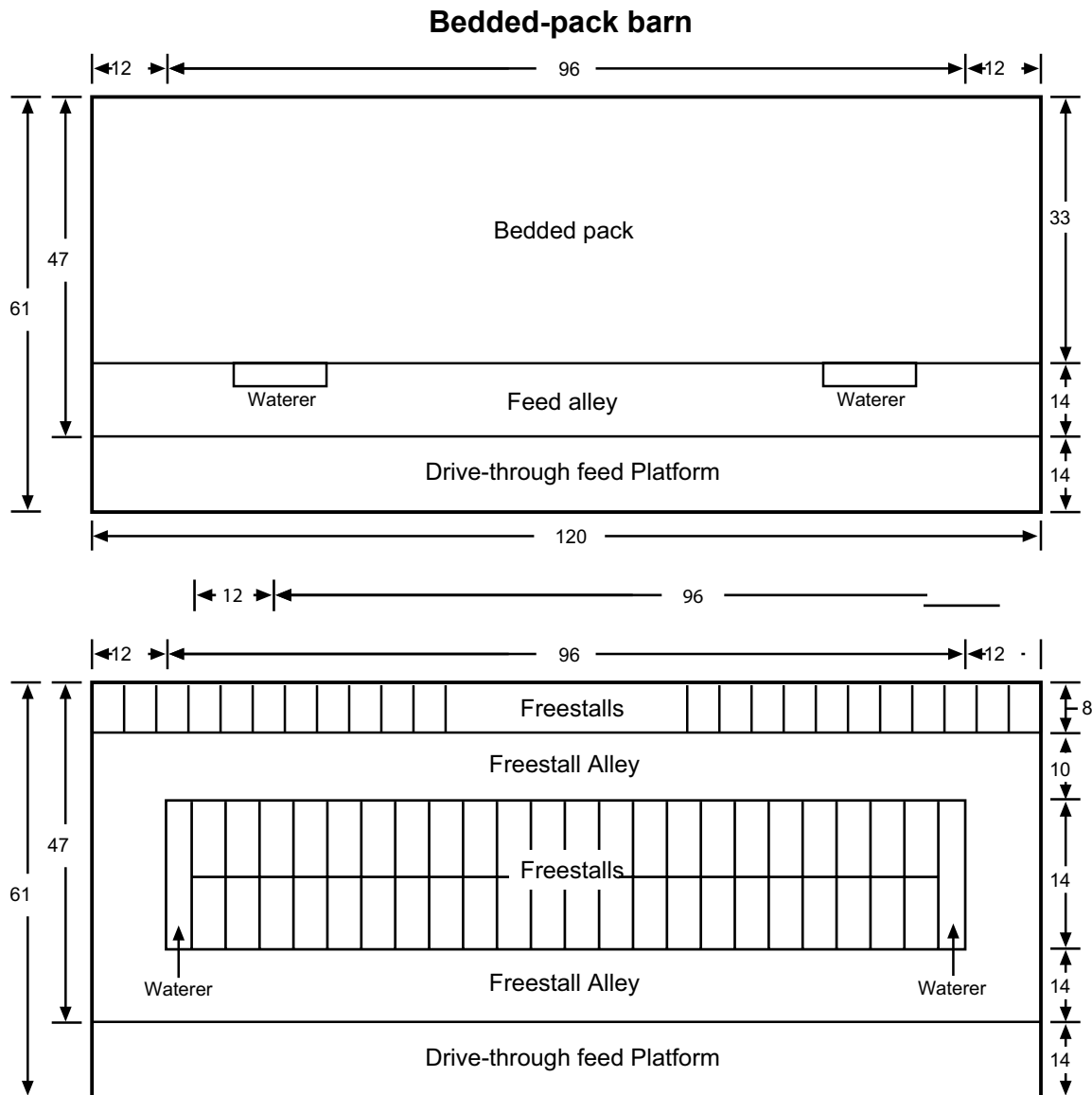
Figure 3. A bedded-pack barn (top) based on the plan for a 3-row, drive-through freestall barn (bottom). The bedded-pack barn would house 39 cows; the freestall barn would house 78 cows. All dimensions are in feet.
