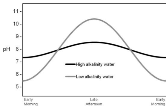
Fig. 1. Changes in pH during a 24-hour period in waters of high and low total alkalinities (Wurts and Durborow, 1992).
